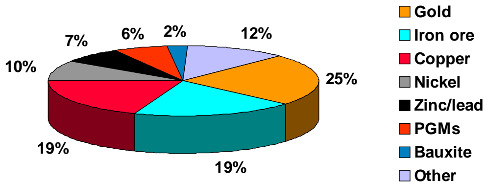
Fig 2. Shares of metallic commodities. World total of all metallic minerals mining (value of metals contained) amounts about 125 billion US$ per annum (2003). PGM, sum value of platinum group metals; bauxite value of the major aluminium mineral production. Source: Raw Materials Data, RMG, Stockholm 2004.
